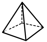
Square Pyramid
