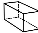
Rectangular Prism
